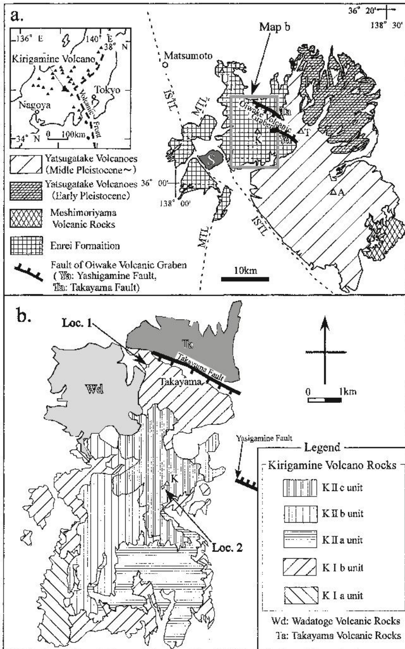
Fig. 1. a) Simplified geological map of Quaternary volcanic products in and around the Suwa and Yatsugatake areas. This map is simplified after Nakano et al. (1998), Ozaki et al. (2002) and Yamada et al. (1989). b) Simplified geological map of the Kirigamine Volcano, the Wadatoge Volcanic Rocks and the Takayama Volcanic Rocks. These Volcanic Rocks compose the upper Enrei Volcanic Rocks (Compilation Group of Natural History in Suwa, 1975). This map simplified after Compilation Group of Natural History in Suwa (1975) and Teshima and Kawachi (1994). Sampling localities for K-Ar dating are also shown. S: Suwako (Suwa Lake), U: Mt. Utsukushigahara, A: Yatsugatake (Mt. Akadake), T: Mt. Tateshinayama, K: Mt. Kurumayama, ISTL: Itoigawa-Shizuoka Tectonic Line active fault system, MTL: Median Tectonic Line.
