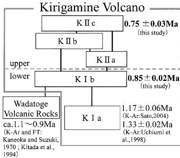
Fig. 2. Stratigraphic relationship of Quaternary volcanic products in the Kirigamine Volcano and the Wadatoge Volcanic Rocks, modified from Compilation Group of Natural History in Suwa (1975).
